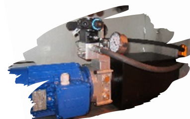
Headbox hydraulics
