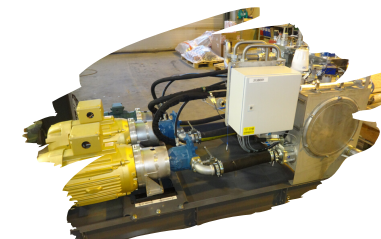
Calander hydraulics
